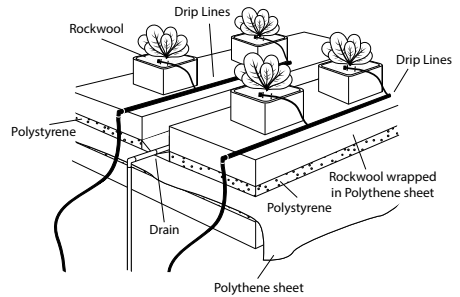
Rockwool culture
